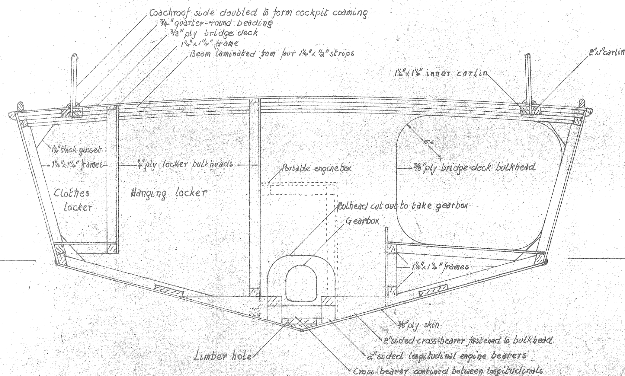
FORWARD SIDE OF BULKHEAD ON STATION 11
