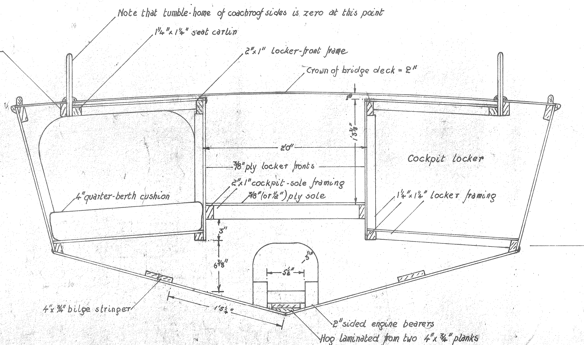
AFT SIDE OF BULKHEAD ON STATION 11
