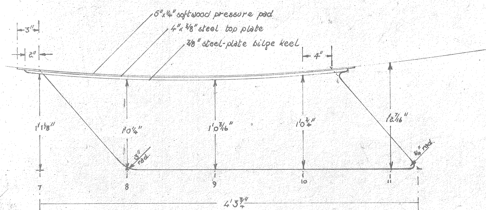
PROFILE OF BILGE KEEL
