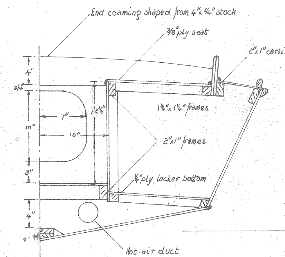
HALF OF FORWARD SIDE
