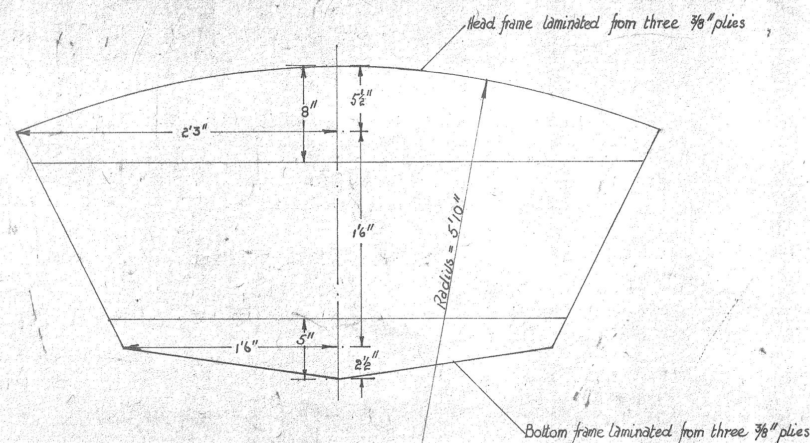
EXPANSION OF TRANSOM
