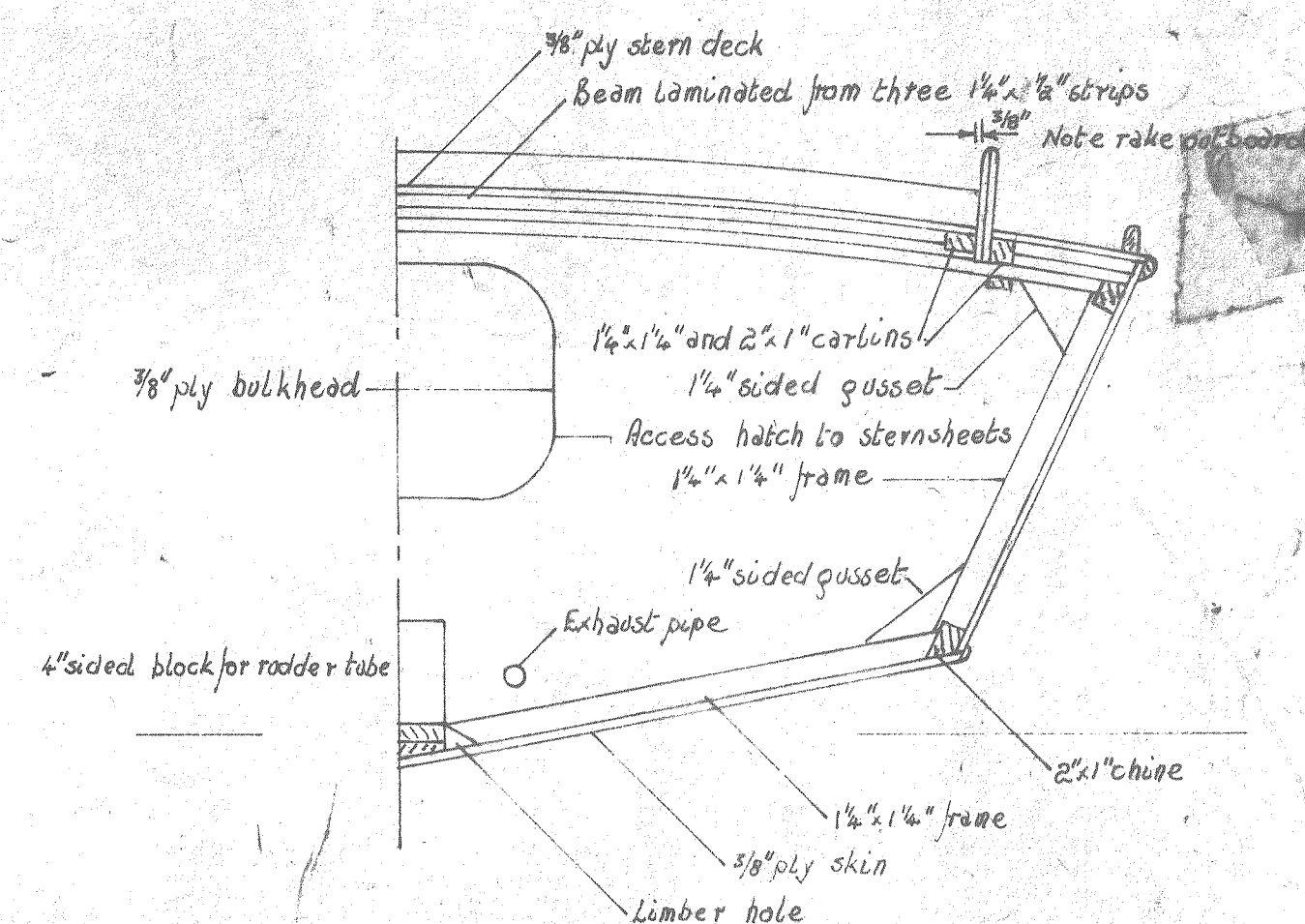
HALF OF AFT SIDE BULKHEAD ON STATION 14A
