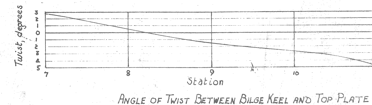
ANGLE OF TWIST BETWEEN BILGE KEEL AND TOP PLATE
