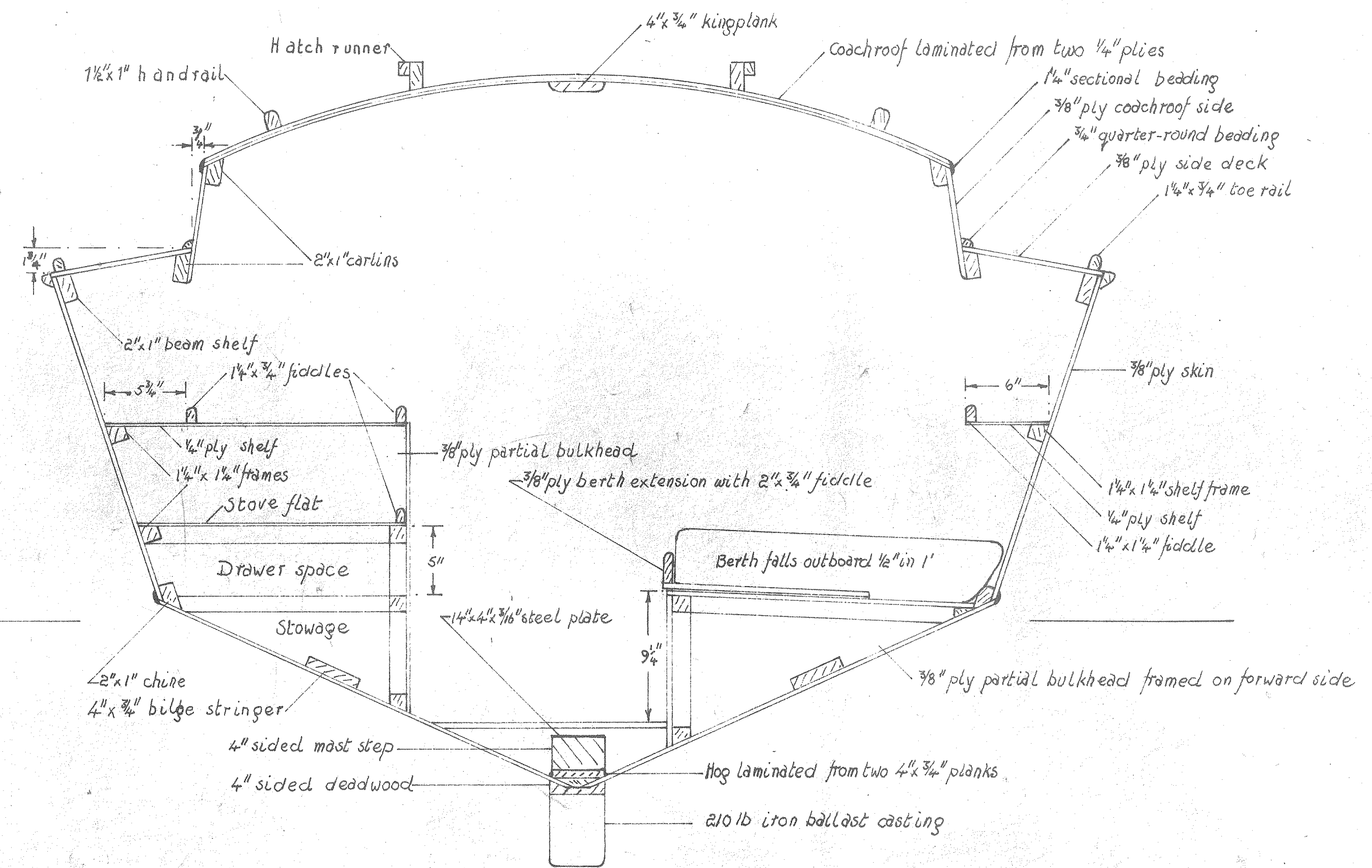
PARTIAL BULKHEADS ON STATION 6A
