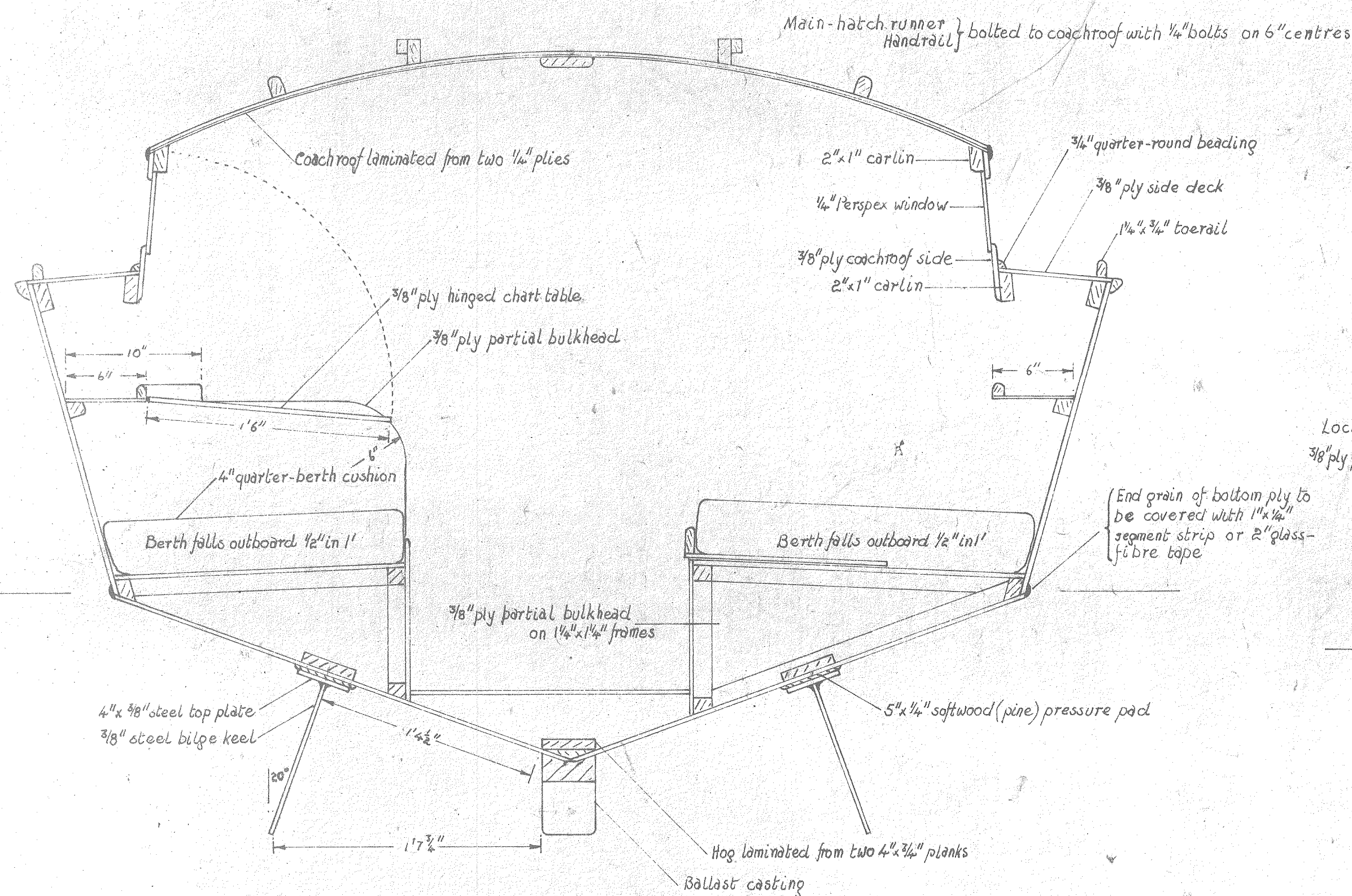
AFT SIDE OF PARTIAL BULKHEADS ON STATION 8A
