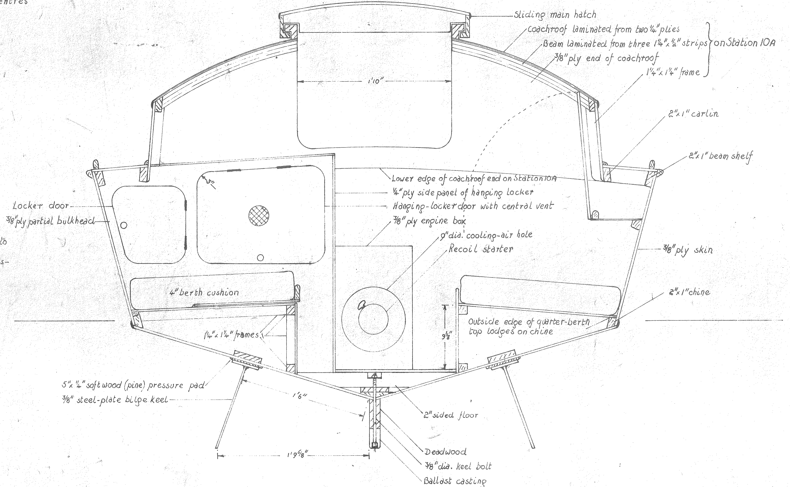
LOOKING AFT ON STATION 10
