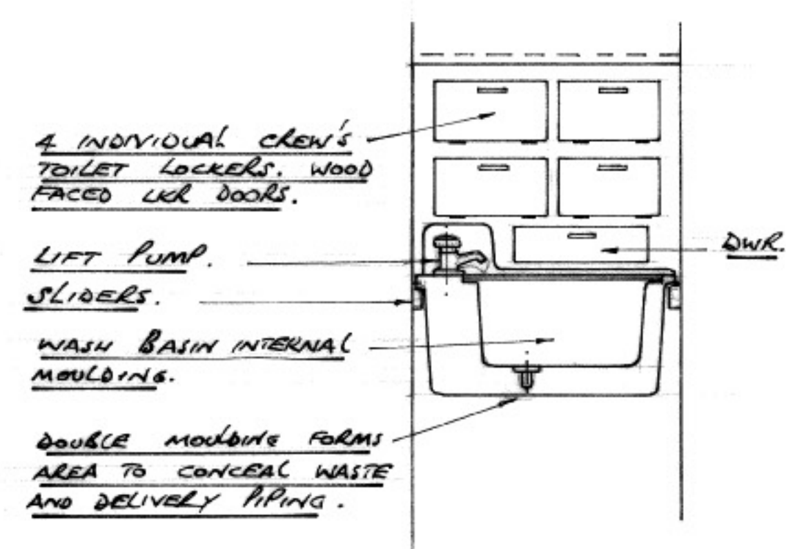
FACE ELEVATION OF WASH UNIT.
