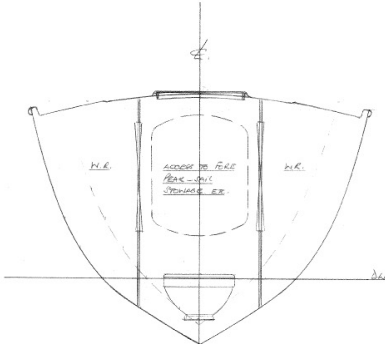
SECTION AT 2 THROUGH TOILET. LOOKING FWD.
